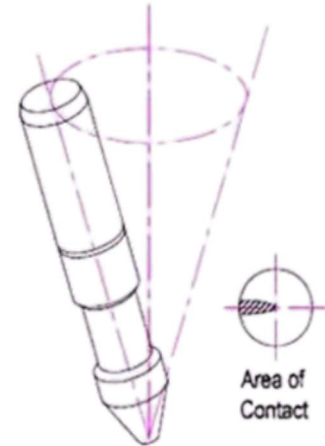
Orbital Riveting Process
